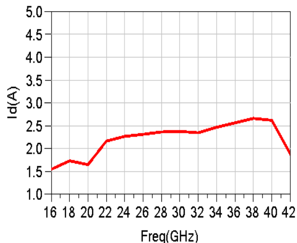
饱和电流vs.频率@Pin= 24 dBm
